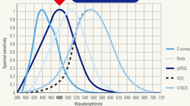
Sensitivity curve of melanopsin (ipRGC)
