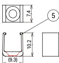
Mounting clip for RIMiT kk (LRMCK-PT-C) 5pcs/1bag
