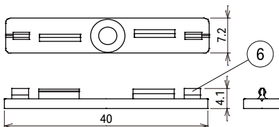
Mounting clip D (LRM-PT-D) 5pcs/1bag
