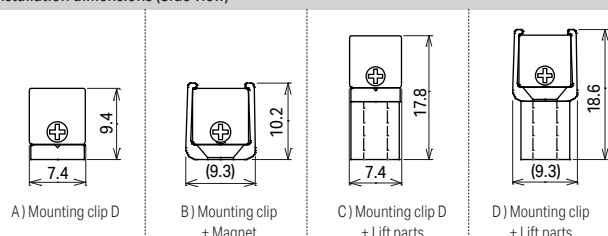
Installation dimensions (Side view)
