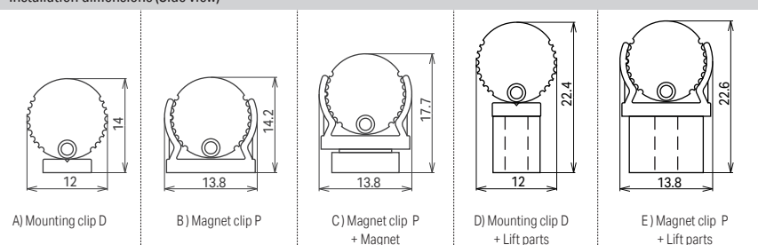
Installation dimensions (Side view)
