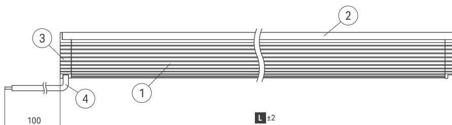
Installation dimensions (Side view)
