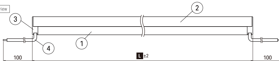
Installation dimensions (Side view)
