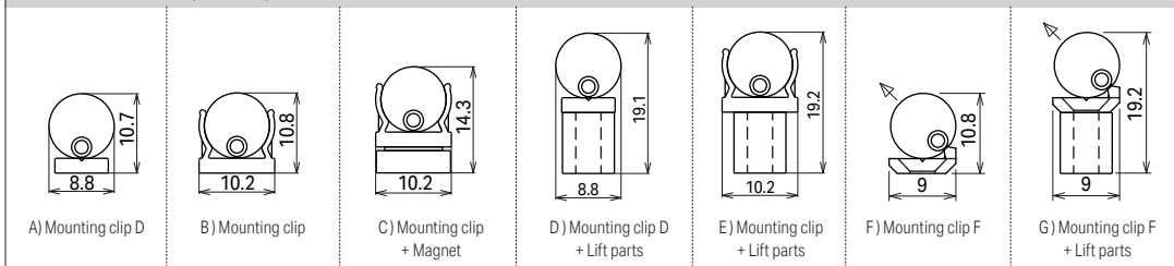
Installation dimensions (Side view)
