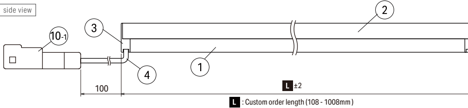
Installation dimensions (Side view)
