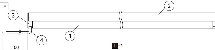
Installation dimensions (Side view)
