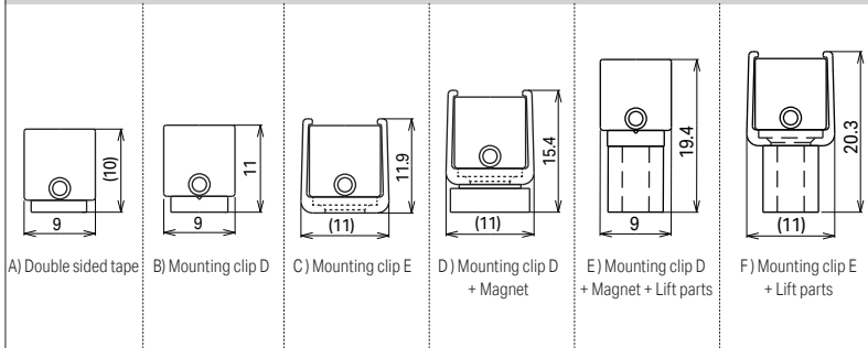
Installation dimensions (Side view)
