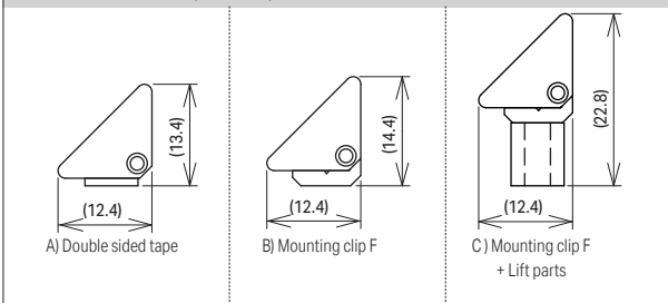
Installation dimensions (Side view)
