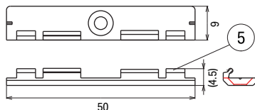
Mounting clip F (LRM-PT-F) 5pcs/1bag
