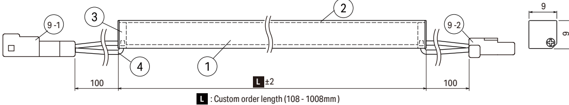
Installation dimensions (Side view)
