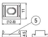
Mounting clip for RIMiT us (LRMUS-PT-A) 5pcs/1bag
