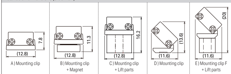
Installation dimensions (Side view)
