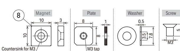
Magnet set A (MG-A) 5pcs/1bag
