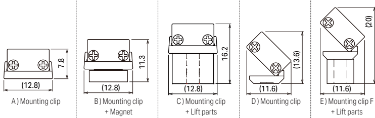
Installation dimensions (Side view)
