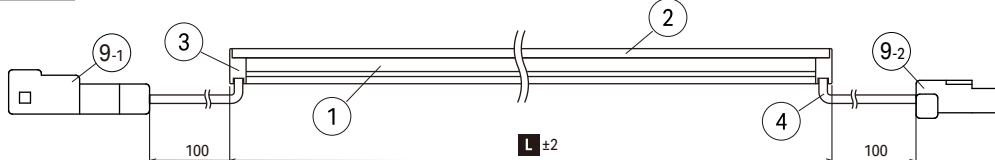
side view
