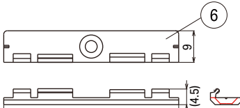
Mounting clip F (LRM-PT-F) 5pcs/1bag
